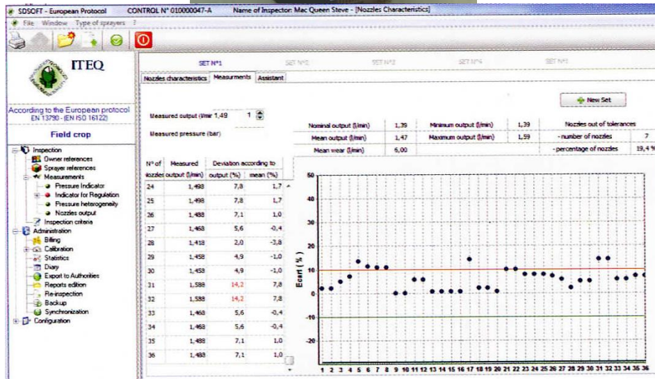
Figure 6.1. A device of ITEQ company for testing intensity of liquid outflow from agricultural atomizers and an exemplary protocol of these tests
