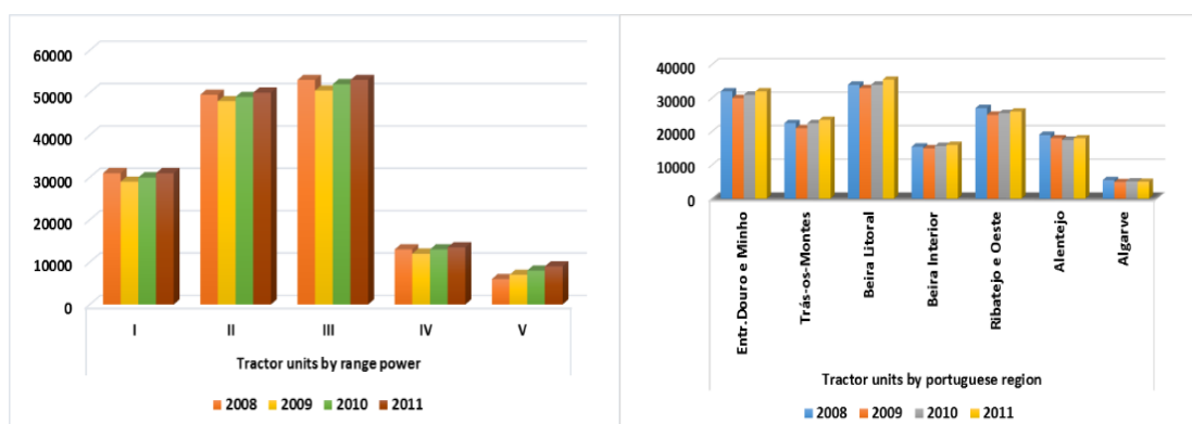
Figure 5.2. Distribution of tractors by engine power (class I – 35hp; class II- 35 to 50hp; class III – 50 to 80hp; class IV – 80 – 100; class V- >100hp) (left) and region (right) in the period of 2008-2011 (DGADR, 2014)
