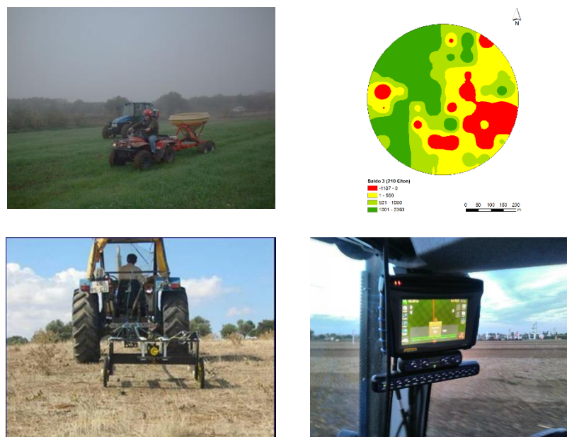
Figure 5.4. The use of an ATV, Yield mapping, tractors data management and guidance systems operations are some examples of the implementation of sustainable smart strategies of mechanization
