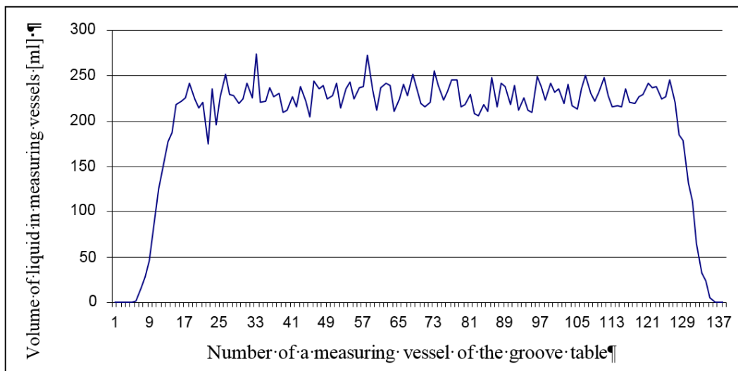
Figure 6.6. Characteristics of nozzle liquid fall obtained on a virtual groove table of grooves 100 mm wide for the sprayer XR 110 VK with the pressure of 3 bars. CV =6,43 %
