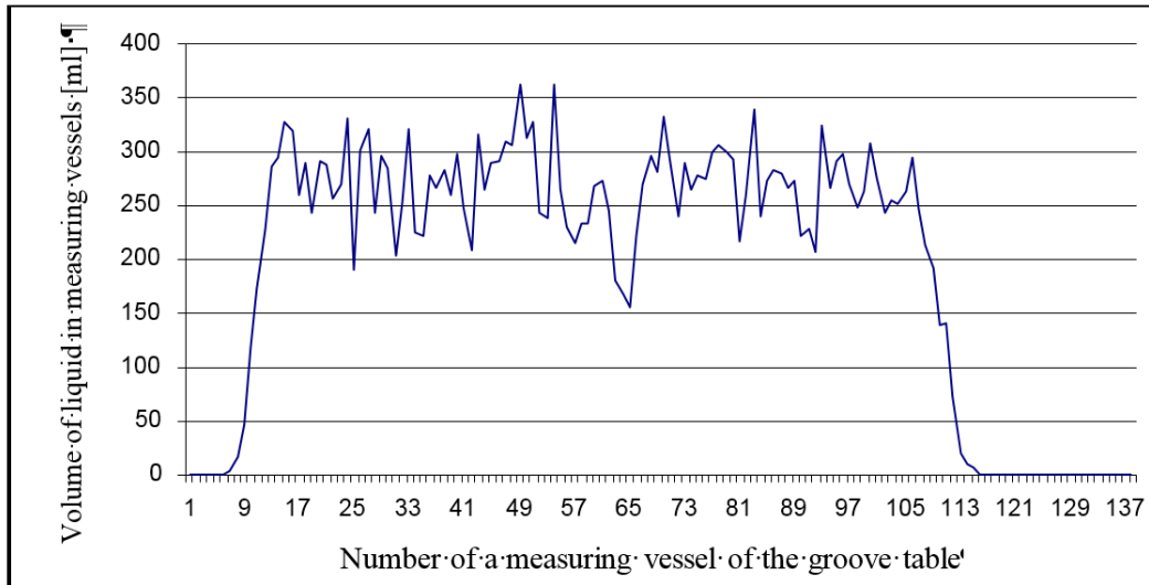
Figure 6.7. Characteristics of nozzle liquid fall obtained on a virtual groove table of grooves 100 mm wide for the sprayer TTD JET RS 110 R with the pressure of 3 bars. CV =15 %
