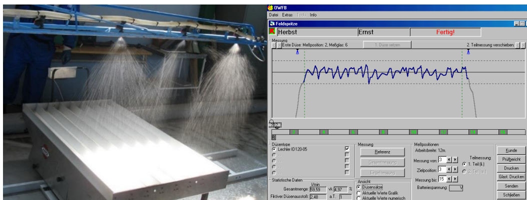
Figure 6.2. The electronic groove table for testing uniformity of distribution of atomized liquid fall and a protocol from these tests
