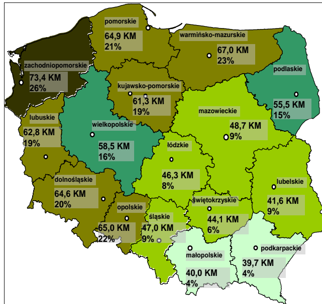
Figure 7.2. Average tractor power in Polish provinces in 2010 (in HP (KM), % tractors over 100 HP)
