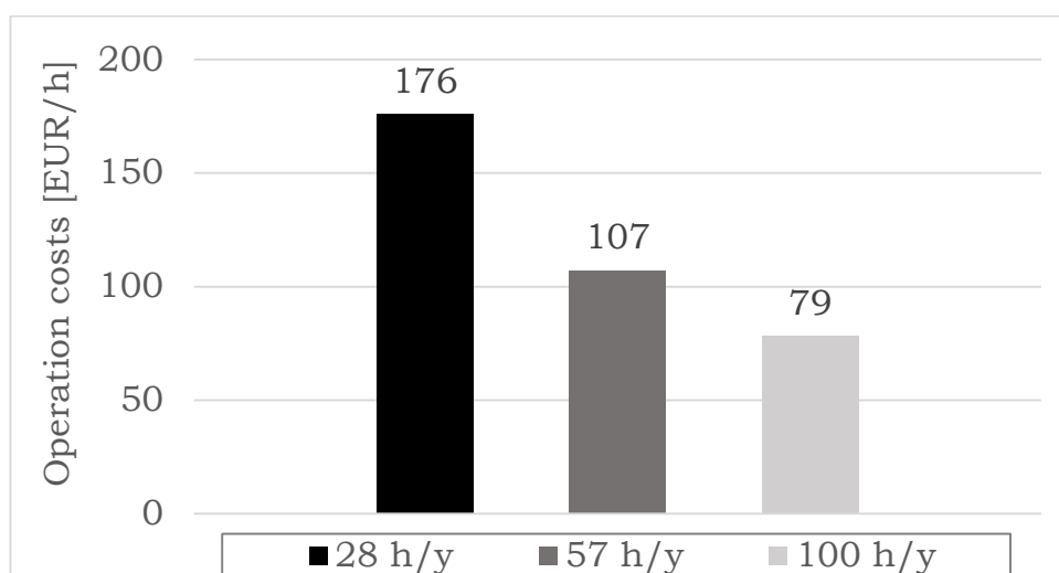
Figure 7.4. Changes in the unit operation costs (in euro per hour) of combine harvester as a function of yearly usage (hours per year)
